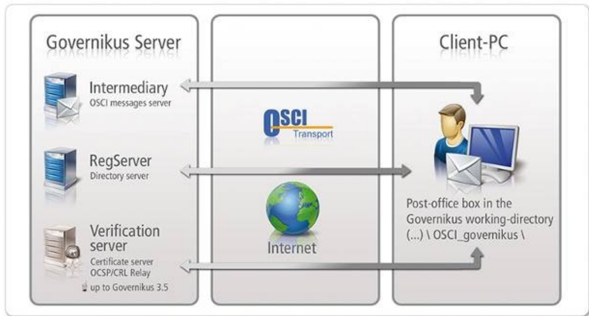
Figure 1: Data traffic between client and server
