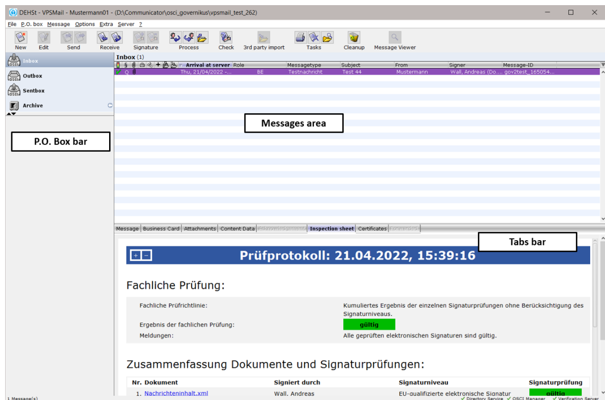
Figure 2: User interface
