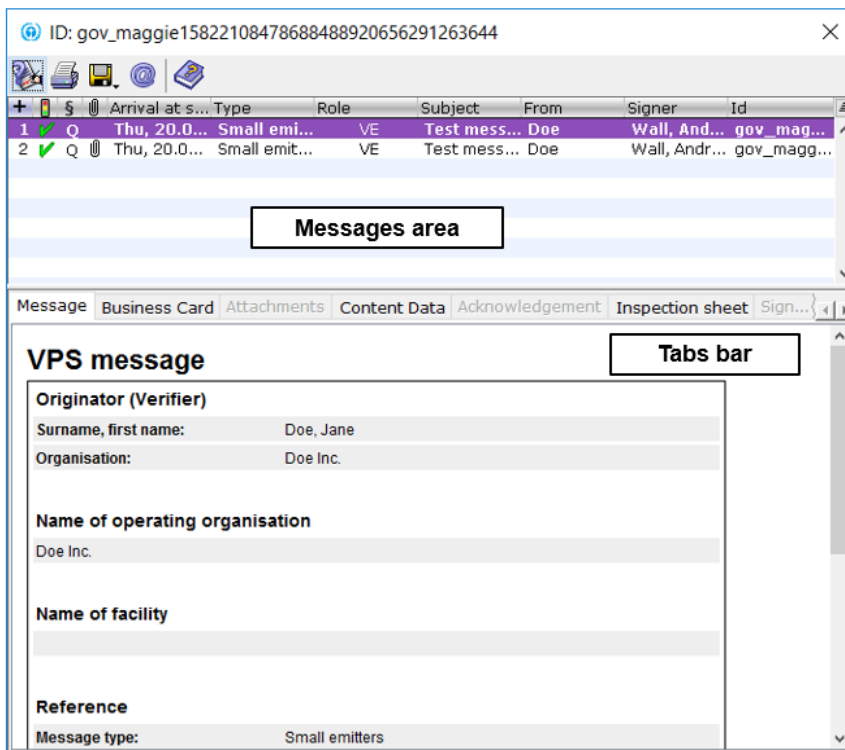
Figure 22: Message Viewer
